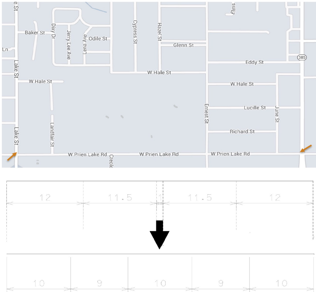
Figure 2.8. LA 1138 layout and lane configuration (before and after)
