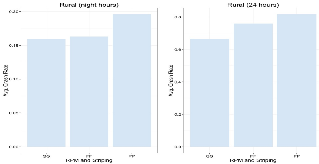
Figure 4.2. Average crash rate by different ratings on rural freeway
