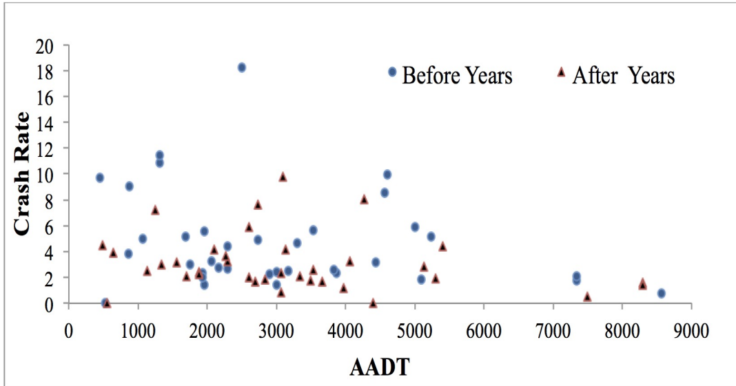
Figure 3.6. AADT vs. crash rate in before-after periods
