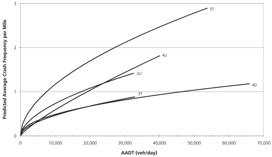
Figure 2.13. Safety Performance Function (SPF) for ROR crashes
