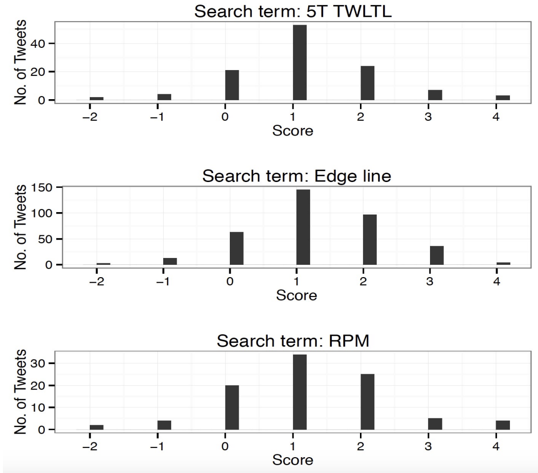
Figure 5.4. Sentiment score
