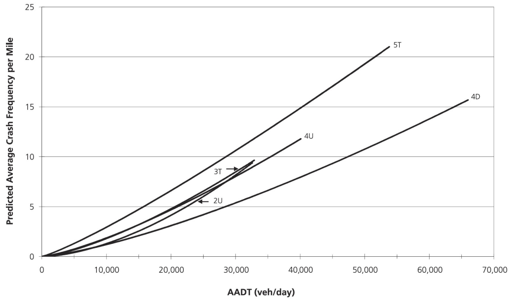
Figure 2.14. SPF graphics for multiple vehicle non-driveway collisions
