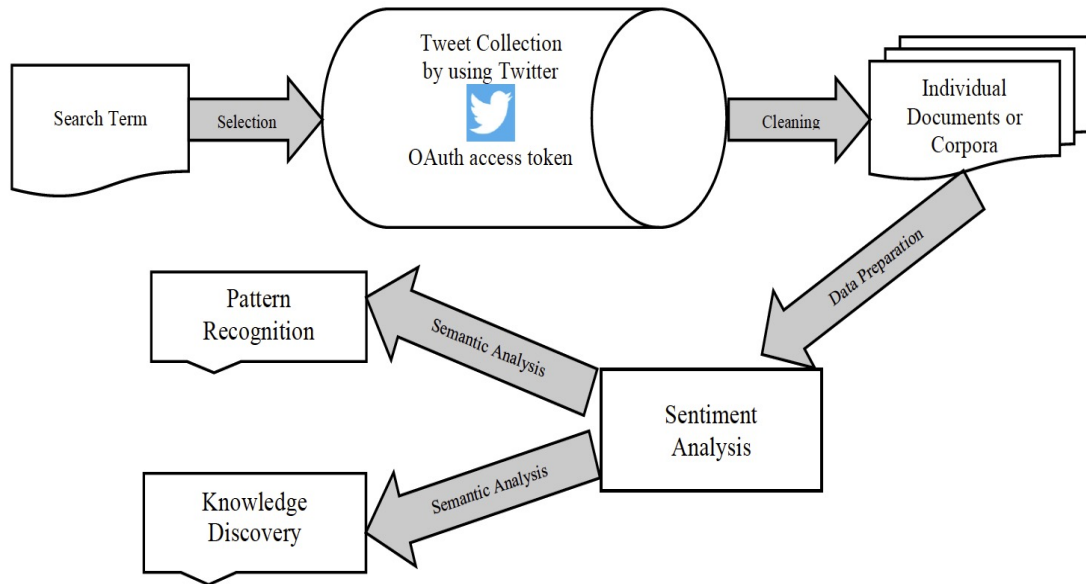
Figure 5.3. Twitter mining
