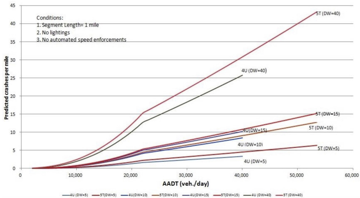
Figure 2.15. Multiple-vehicle driveway-related predicted crashes per mile
